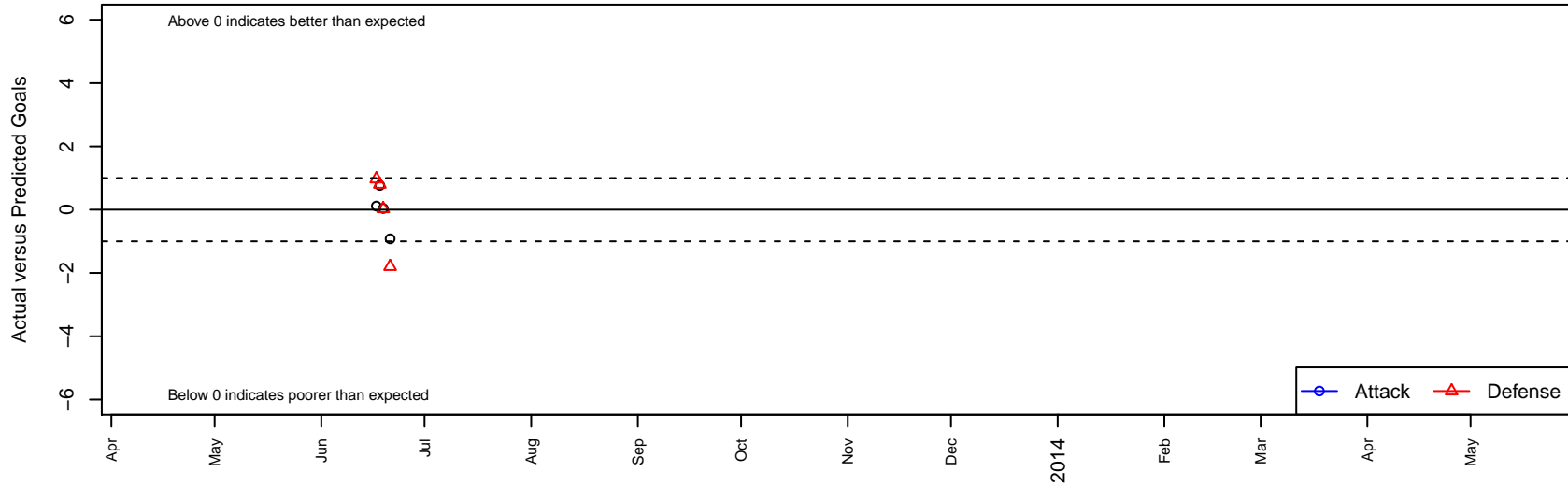
Utah FC 97 MA B96 Dots are actual minus expected GF (blue circles) and GA (red triangles). Blue line is smoothed change in attack strength. Red is smoothed change in defense strength.
